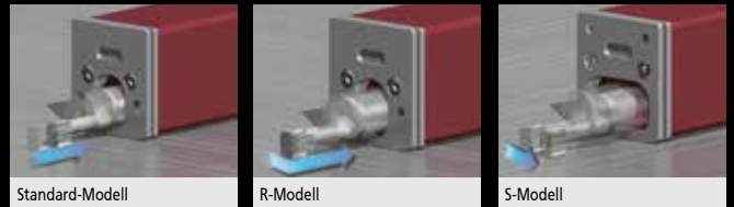
Standard-Modell
